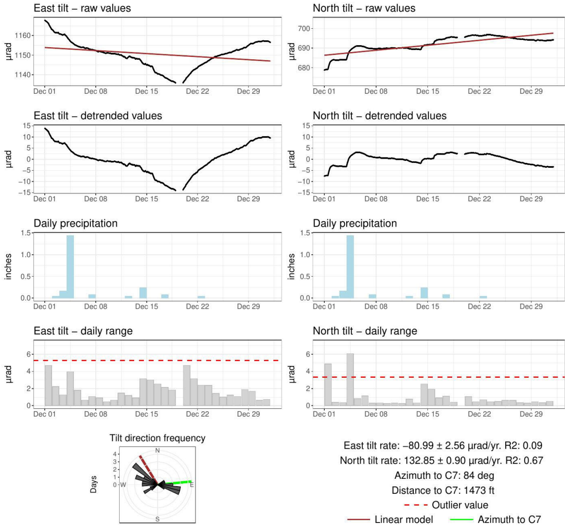
Figure 3. SD11 tilt signals for the current monthly reporting period, showing changes in the east-component tilt direction following maintenance on December 19.
