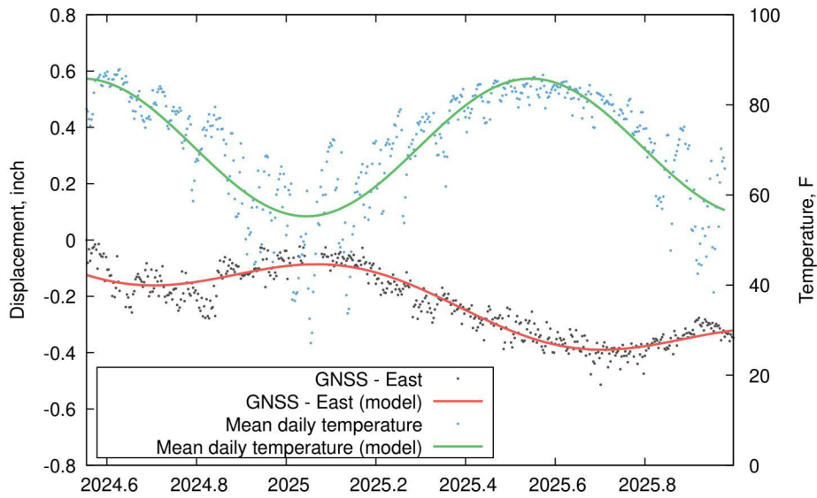
Figure 6. REMNE east deformation component and its cyclical model superimposed on the linear trend (red), alongside mean daily temperature and its cyclical model (green). Seasonal variations show eastward trends during cold periods and westward trends during warm periods.
