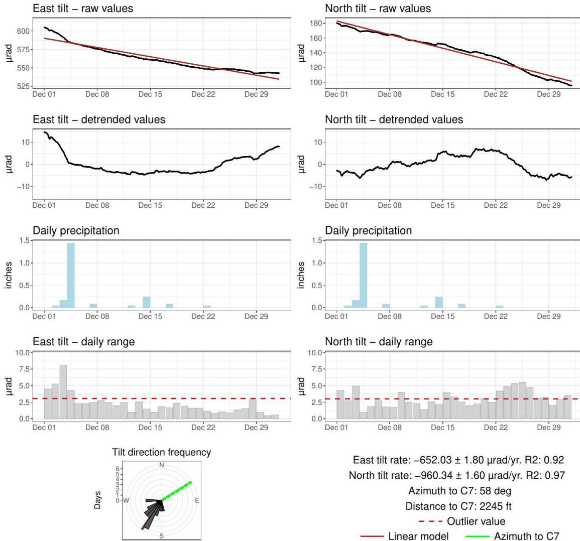
Figure 5. SSD19 tilt signals for the current monthly reporting period, showing periodically elevated rates in the east and north components.
