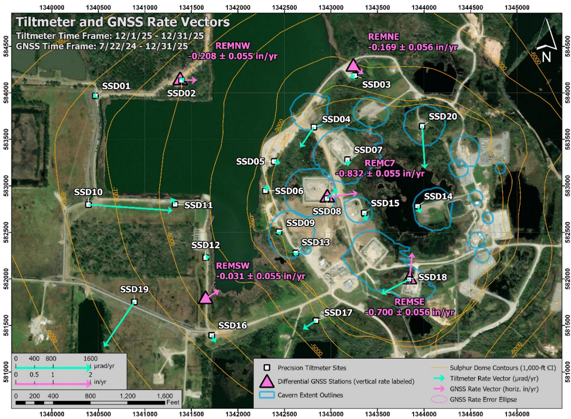
Figure 9. Map of deformation rate vectors for the tiltmeters and GNSS stations over their respective evaluated time frames. The tiltmeter vectors are shown in cyan and scaled by their respective values in units of microradians per year. The GNSS vectors and their corresponding error ellipses (derived from east and north rate errors) are shown in pink representing inches of horizontal movement per year. The GNSS stations are additionally labeled with the vertical motion rate and corresponding error value.
