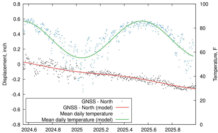
Figure 7. REMNE north deformation component with its cyclical model superimposed on the linear trend (red), alongside mean daily temperature and its cyclical model (green). Seasonal variations in the north component are unnoticeable.
