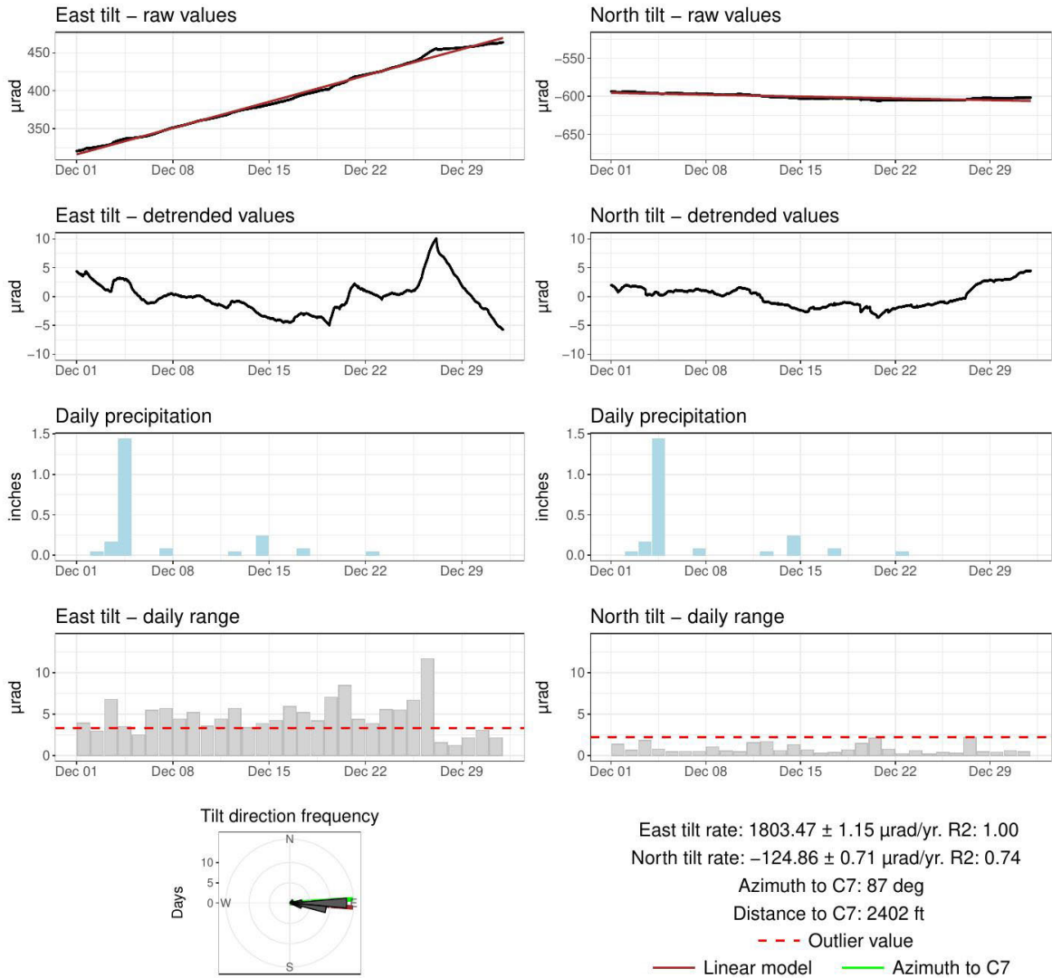
Figure 4. SSD10 tilt signals for the current monthly reporting period, showing an elevated tilt rate in the east component.
