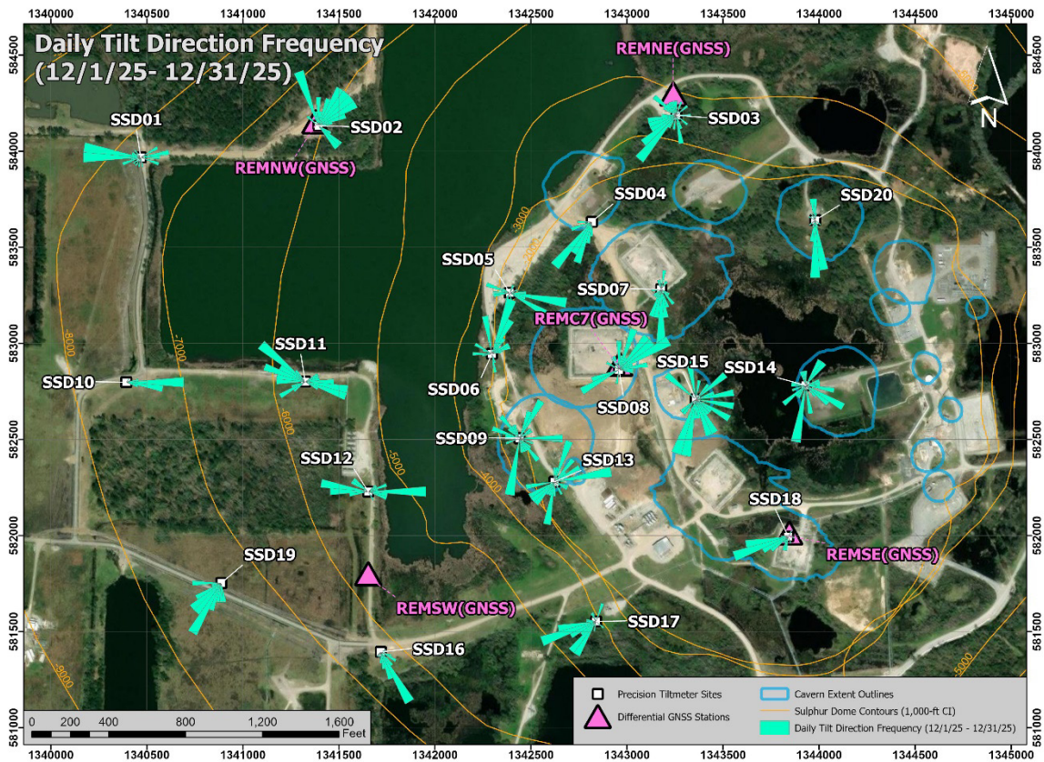
Figure 11. Map of daily tilt direction distribution for each tiltmeter for the current monthly reporting period. Rose diagrams indicate the number of days that tilt was oriented along specific azimuths (bin size is 10°).
