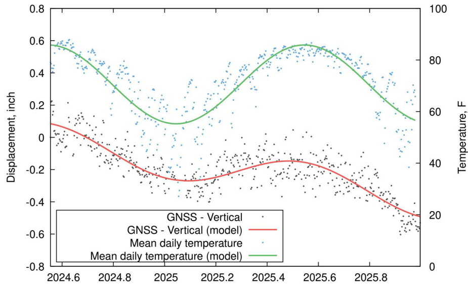
Figure 8. REMNE vertical deformation component with its cyclical model superimposed on the linear trend (red), alongside mean daily temperature and its cyclical model (green). Seasonal variations show downward trends during cold periods and upward trends during warm periods.
