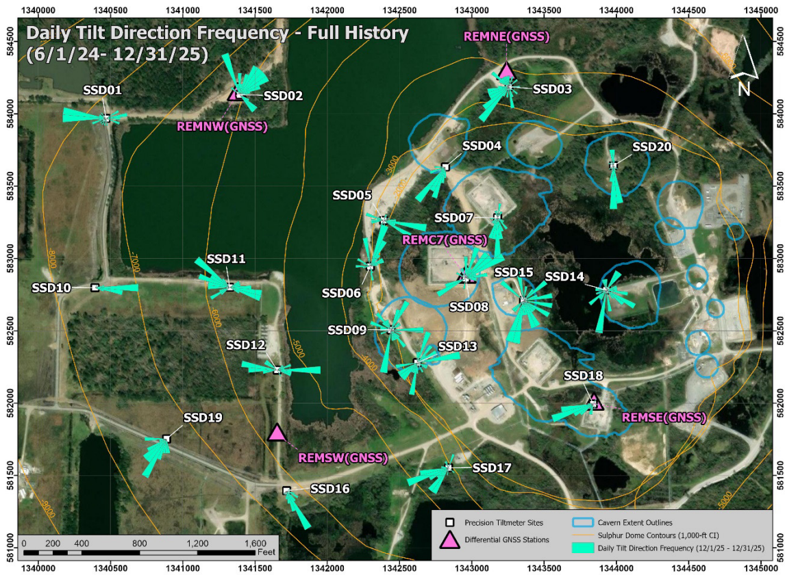
Figure 10. Map of daily tilt direction distribution for each tiltmeter for the full data history beginning in June 2024. Rose diagrams indicate the number of days that tilt was oriented along specific azimuths (bin size is 10°).
