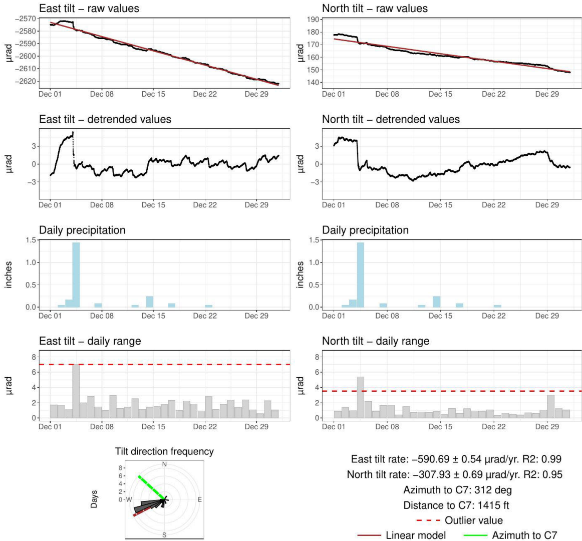
Figure 2. Charts of the tilt signals observed by the SSD18 tiltmeter over the current monthly reporting period. Note the changes in the east and north components in response to a precipitation event on December 4.
