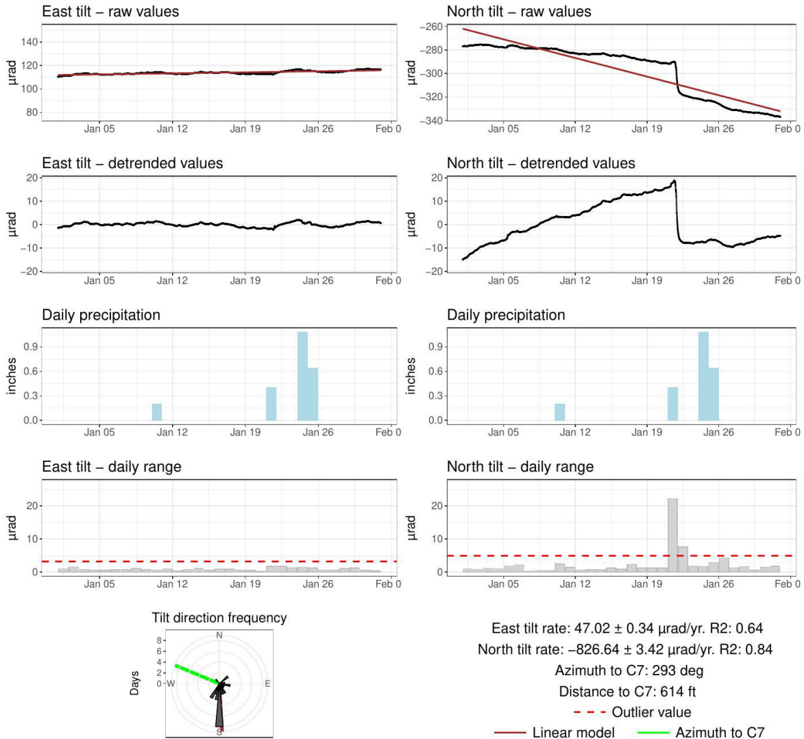
Figure 4. Charts of the tilt signals observed by the SSD15 tiltmeter over the current monthly reporting period, illustrating elevated tilt from January 21-22 in response to precipitation on January 21. Note that the substantial rainfall on January 24-25 did not produce a correspondingly large tilt response.
