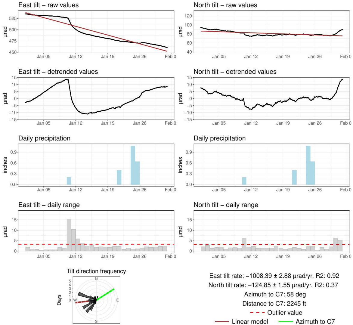
Figure 3. Charts of the tilt signals observed by the SSD19 tiltmeter over the current monthly reporting period, illustrating elevated tilt from January 10-12 in response to precipitation on January 10.
