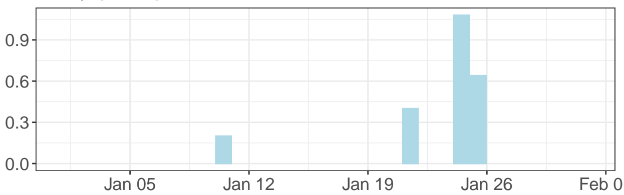
Daily precipitation
