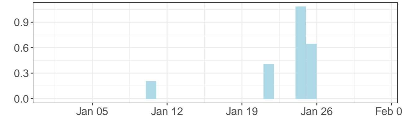
Daily precipitation
