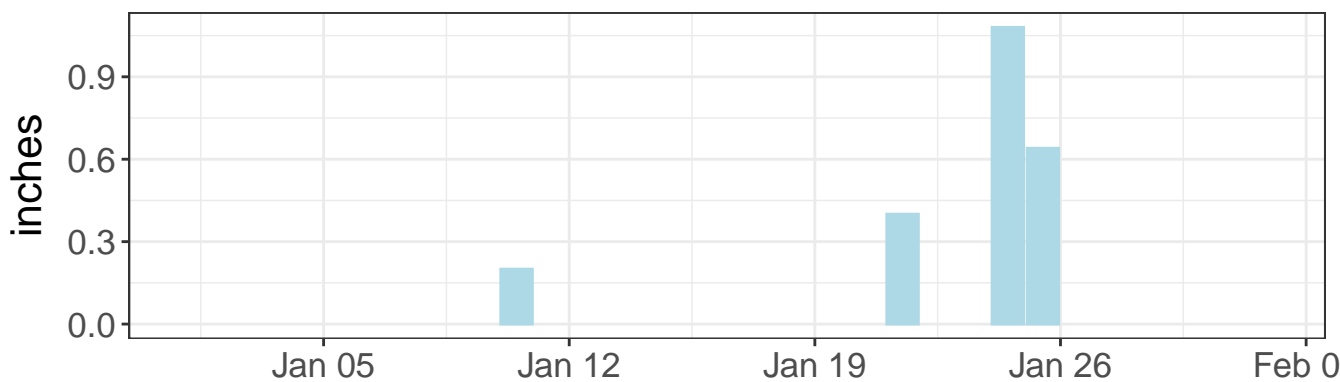
Daily precipitation
