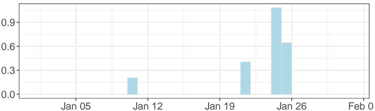
Daily precipitation
