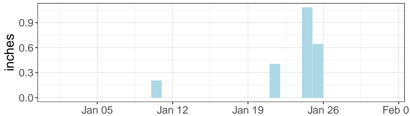
Daily precipitation
