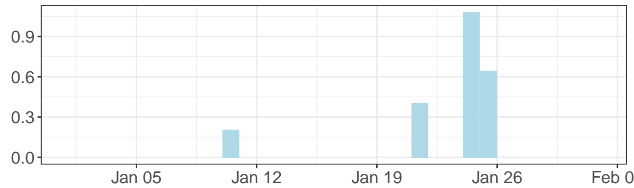
Daily precipitation
