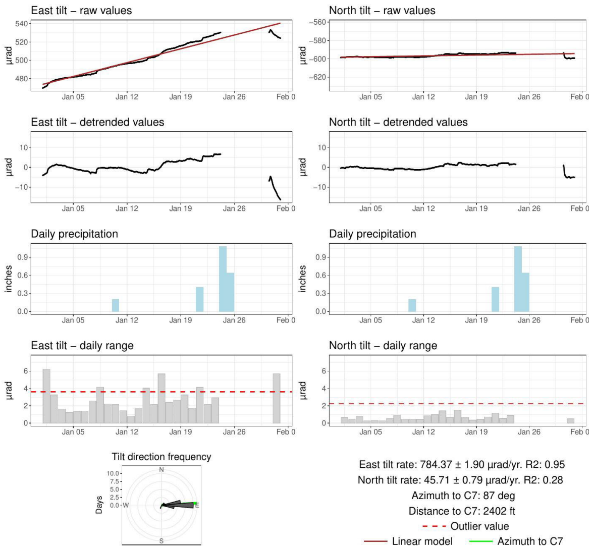
Figure 2. Charts of the tilt signals observed by the SSD10 tiltmeter over the current monthly reporting period. Note that SSD10 was temporarily offline from January 24 to January 30, and following replacement, the tiltmeter required a period of time to stabilize.
