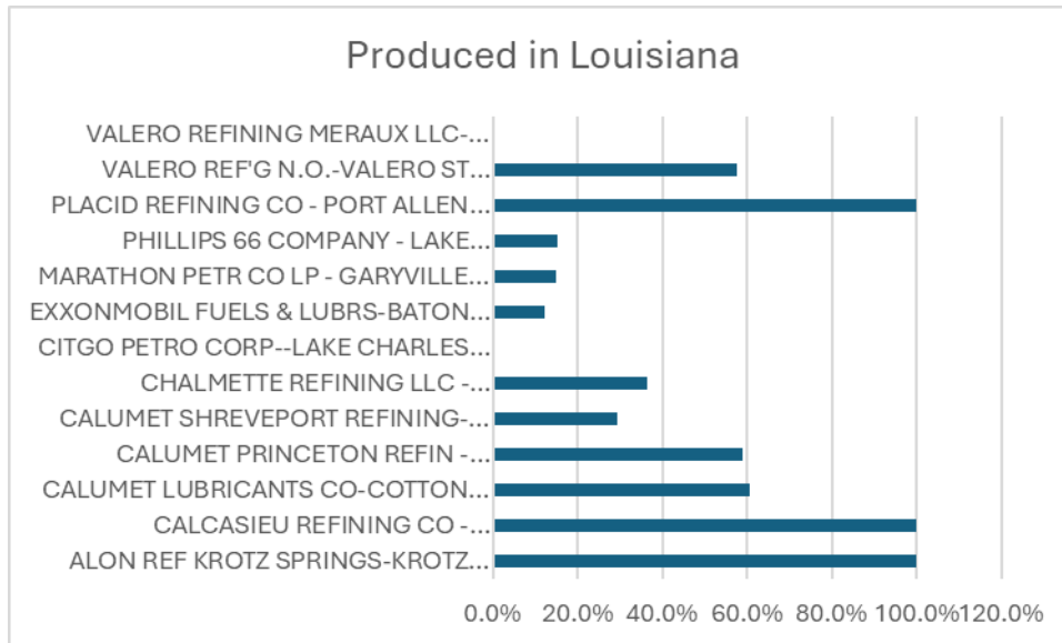
Figure 5 Crude Oil Input Percentages by Source and Refinery 2024 DENR's R3 Report
